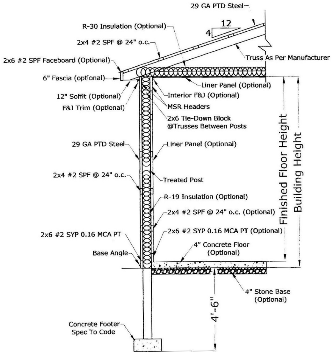
Typical Wall Section No Scale
